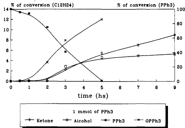
Figure 3. Kinetics of the Gif IV oxidation of cyclododecane ( 6 , 5.0 mmol) in the presence of triphenylphosphine (1 mmol). Experimental conditions: Zn (20.0 mmol), FeCl 2 ·4H 2 O (0.25 mmol), pyridine (28 mL), and acetic acid (2.3 mL). The left ordinate gives the percentages of ketone and alcohol. The right ordinate gives the percentages of triphenylphosphine and triphenylphosphine oxide.
