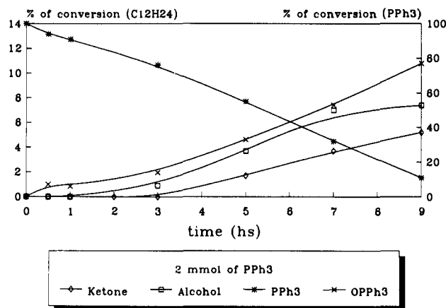
Figure 4. Kinetics for the \text{Gif}^{\text{IV}} oxidation of cyclododecane (6, 5.0 mmol) in the presence of triphenylphosphine (2 mmol). Experimental conditions: Zn (20.0 mmol), \text{FeCl}_2 \cdot 4\text{H}_2\text{O} (0.25 mmol), pyridine (28 mL), and acetic acid (2.3 mL). The left ordinate gives the percentages of ketone and alcohol. The right ordinates gives the percentages of triphenylphosphine and triphenylphosphine oxide.
